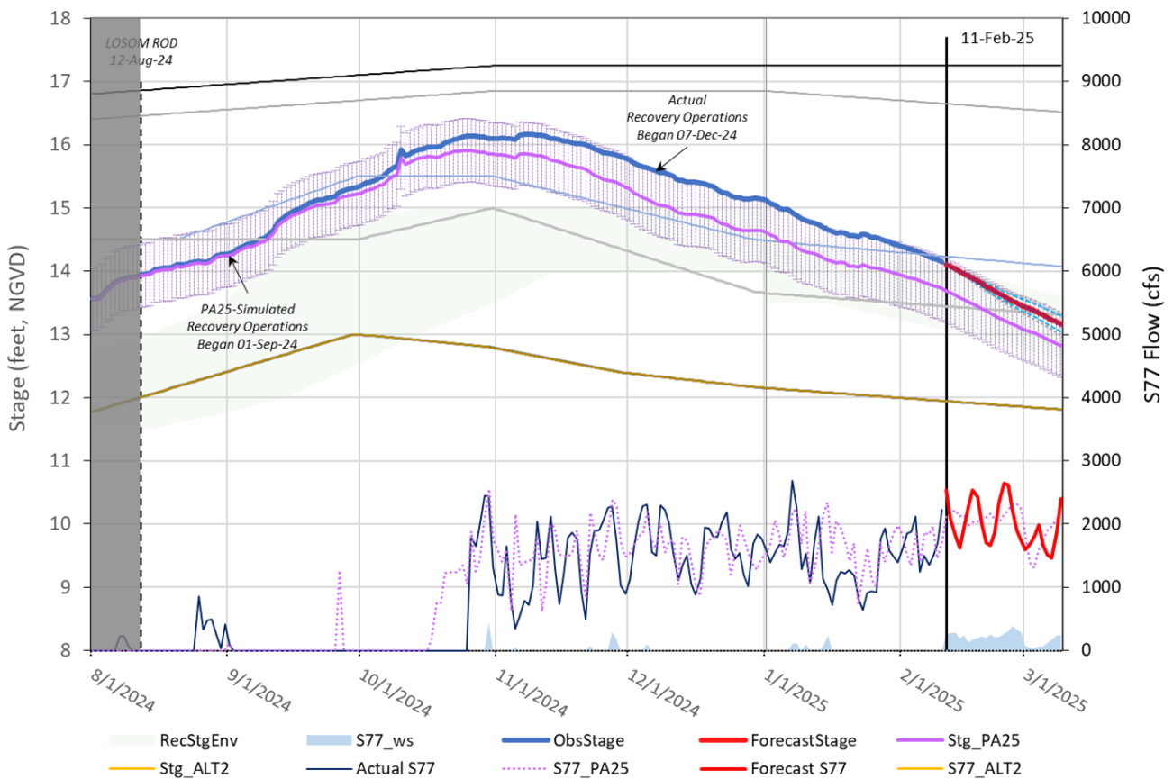
Lake Okeechobee Hindcast & Forecasts* [S79/S80: 2100/1200]
