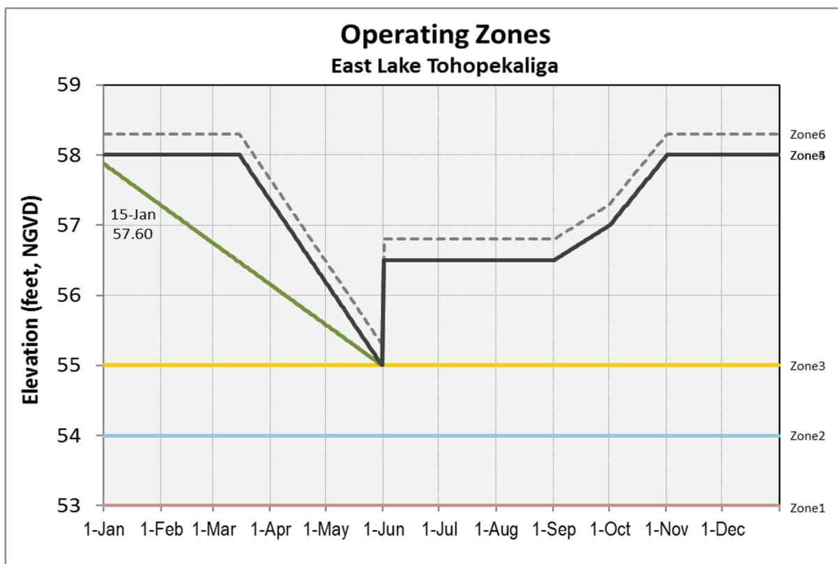
Figure 3-2. East Lake Tohoepkaliga regulation schedule as seen by the UK-OPS Model.
