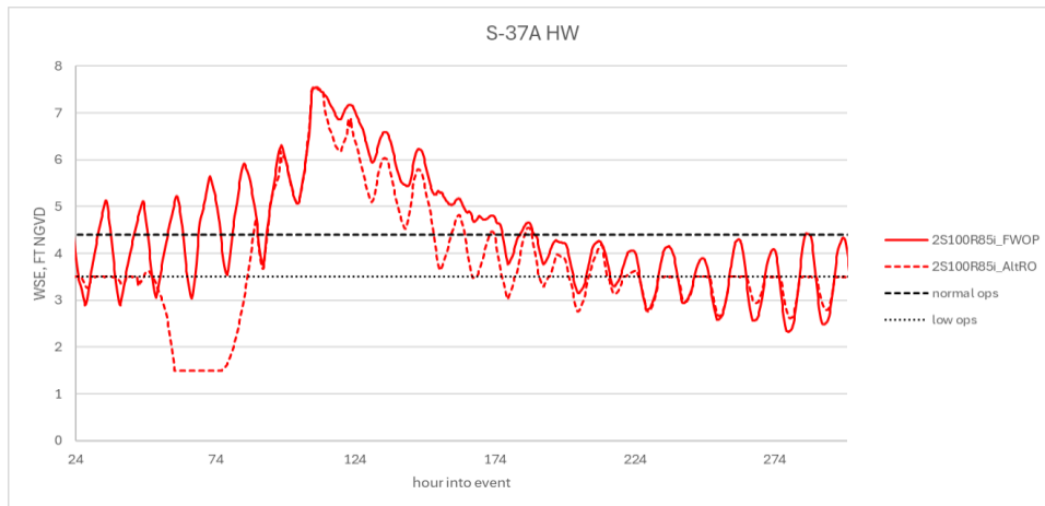
Figure 4-33. Pre-storm Drawdown Prior to Storm Peak.
