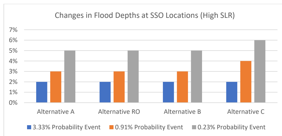
Figure 4-24. Changes in Flood Depths at Sanitary Sewer Overflow Incident Locations, High Sea Level Rise Scenario.
