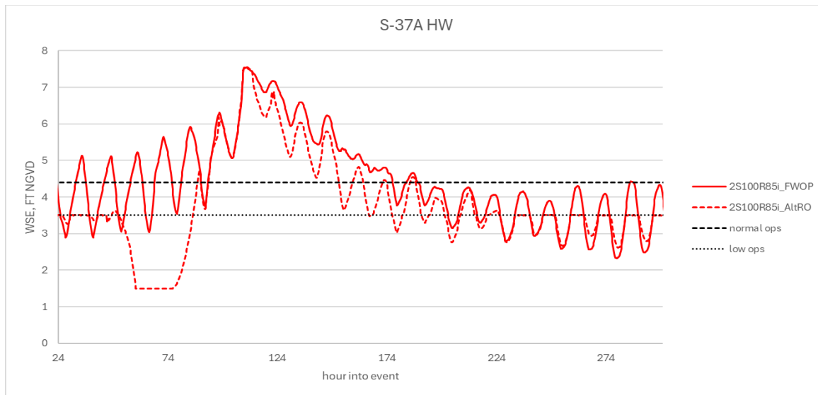
Figure 4-38. Pre-storm Drawdown Prior to Storm Peak.
