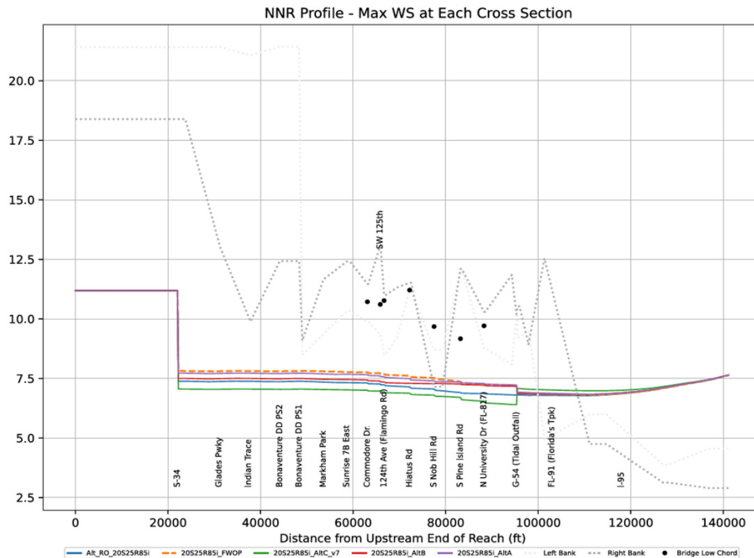
Figure 4-39. Peak Canal Stage Profiles.
