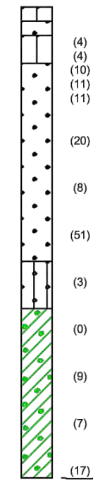
BOR. PZ-06 GROUND ELEV. 28.3
