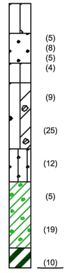
BOR. B-21 GROUND ELEV. 42.7
