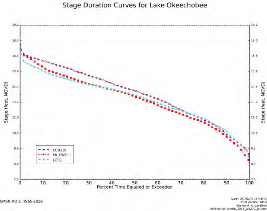
Figure B.1. Lake Okeechobee Stage Duration Curves Comparing LOSOM Baselines and Alternative LCR1.
