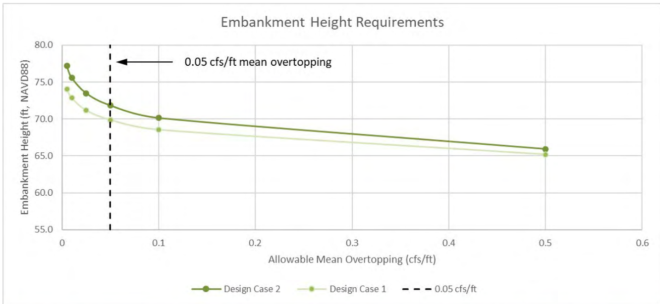
Figure 4. Embankment Height Requirements as a Function of Allowable Overtopping.
