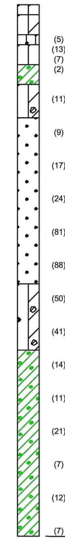
BOR. B-19 GROUND ELEV. 29.9
