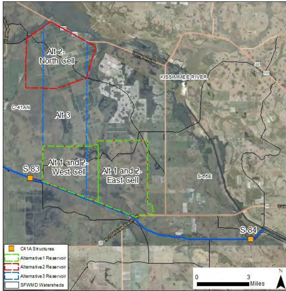
Figure 1. LOCAR Location and Alternatives
