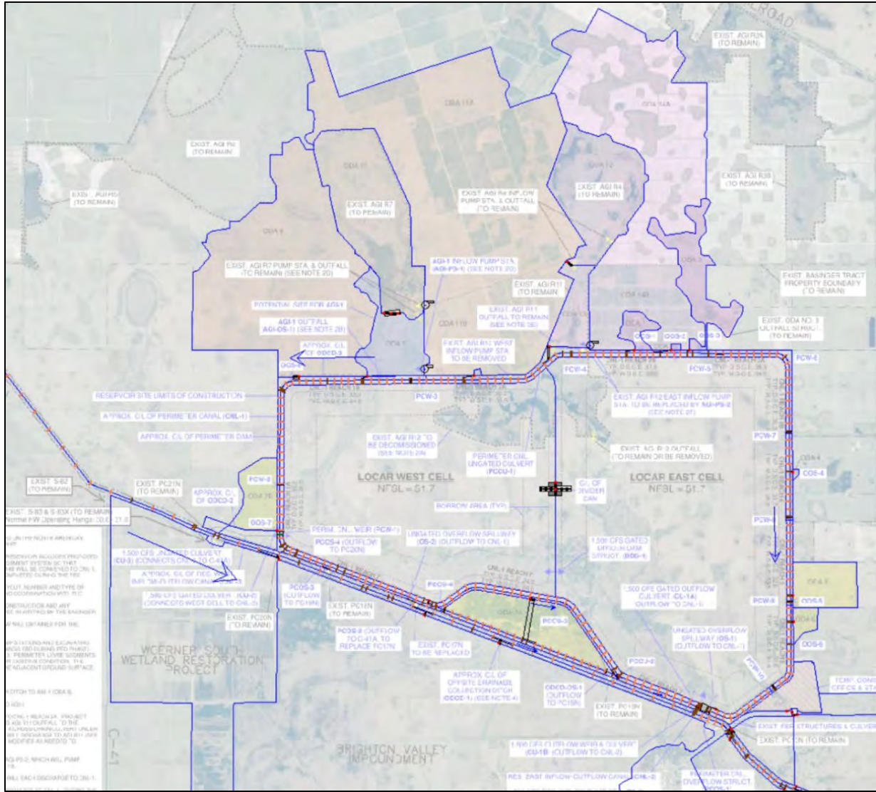
Figure 9. Proposed Condition Model Basins Overlaid on Proposed LOCAR Footprint.
