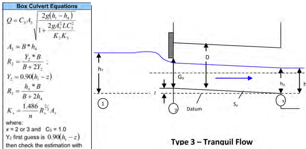
Figure A-1.1-14. Box culvert partial flow equation and diagram.
