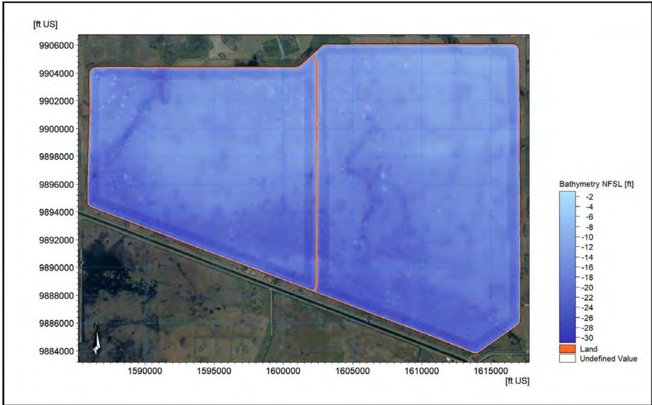
Figure 4-1. Model Bathymetry.
