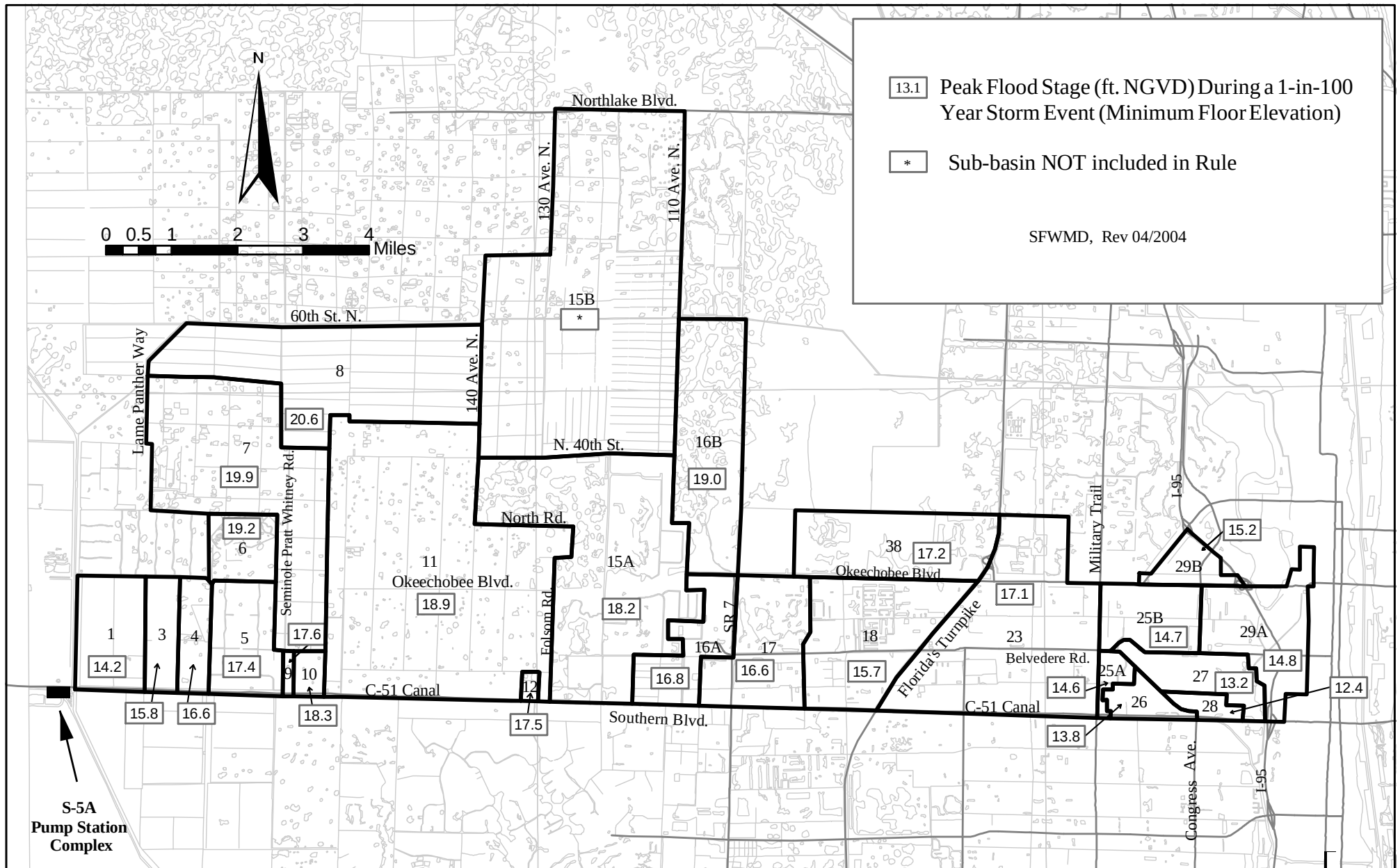
Peak Flood Stage (ft. NGVD) During a 1-in-100 Year Storm Event and Minimum Floor Elevation
