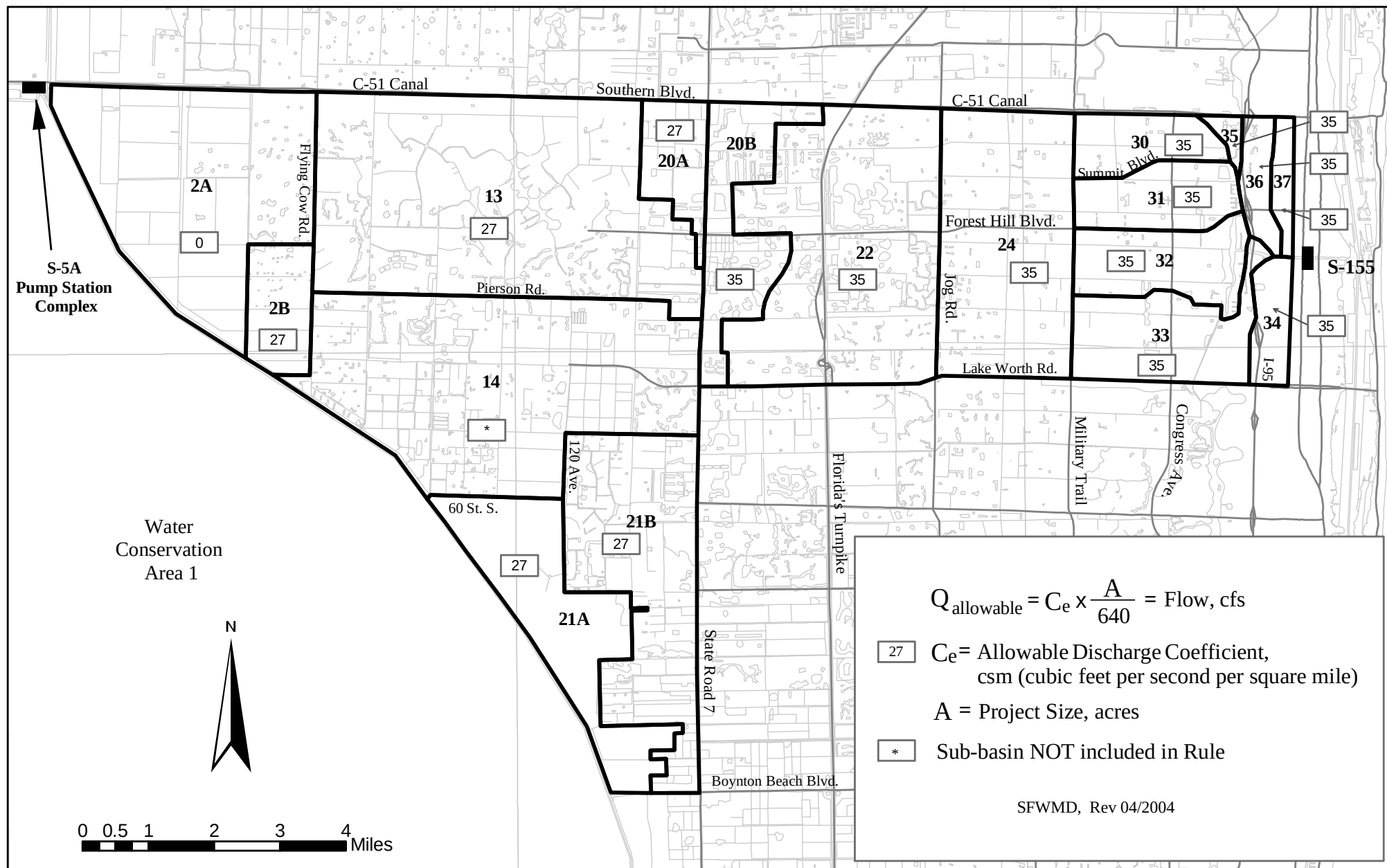
Discharge Coefficients for the Sub-basins of the C-51 Basin in Palm Beach County, Florida
