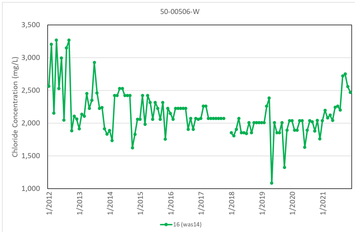
Figure D-32. Chloride concentrations in Town of Manalapan Floridan aquifer system (Avon Park permeable zone) well 16.
