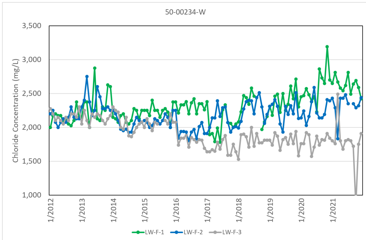
Figure D-31. Chloride concentrations in City of Lake Worth Beach Floridan aquifer system (Avon Park permeable zone) wells LW-F-1, LW-F-2, and LW-F-3.
