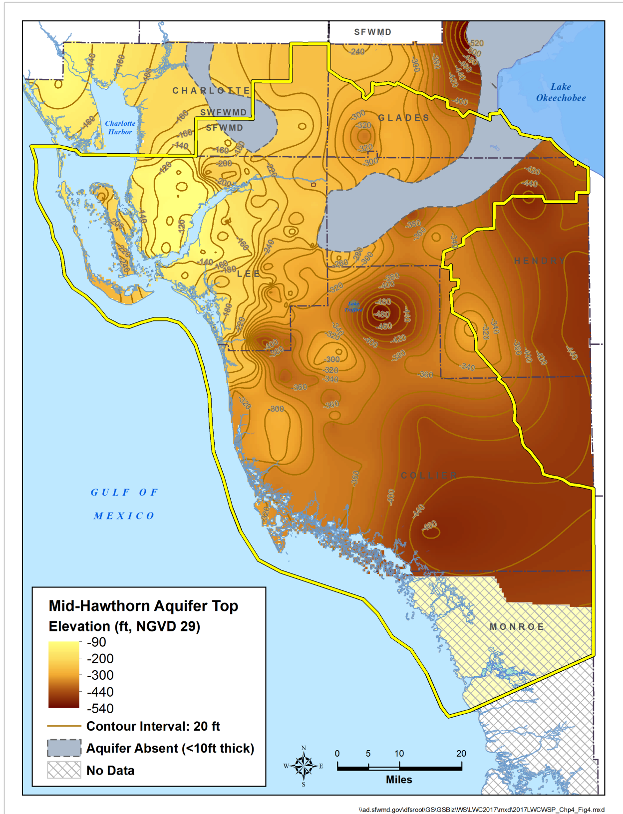
Figure C-8. Structural top (MFL) of the Mid-Hawthorn aquifer in the LWC Planning Area.
