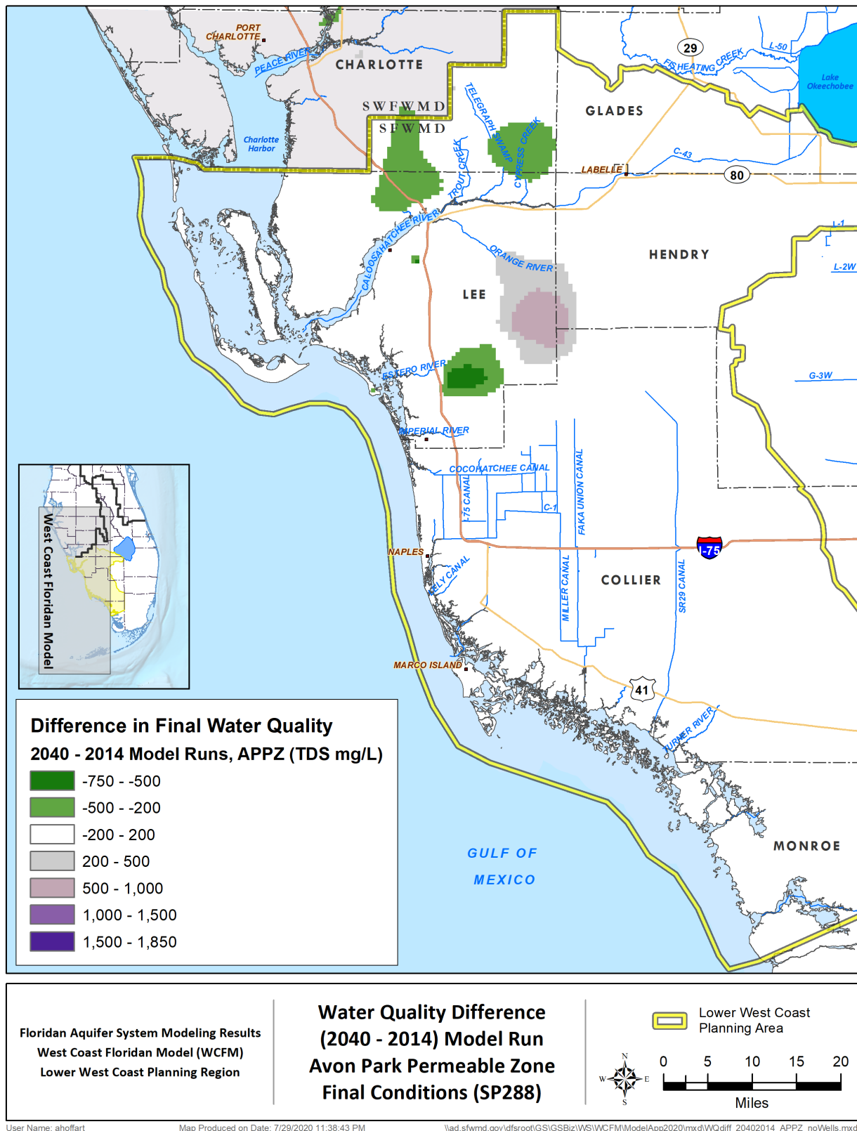
Figure D-31. Avon Park permeable zone water quality (total dissolved solids concentration) difference between 2014 and 2040.
