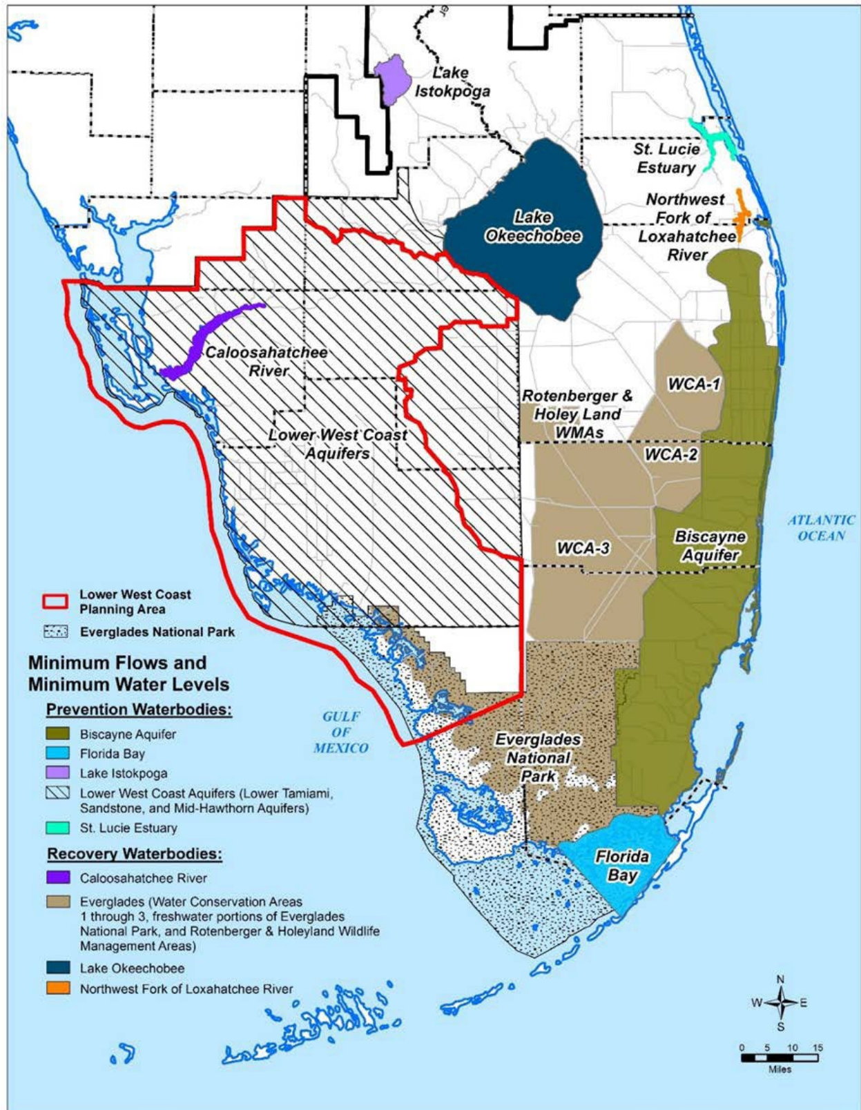
Figure C-1. Adopted minimum flows and minimum water levels in the South Florida Water Management District in relation to the LWC Planning Area.
