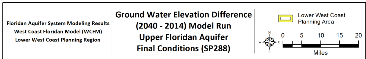
Figure D-22. Upper Floridan aquifer water level differences between 2014 and 2040.
