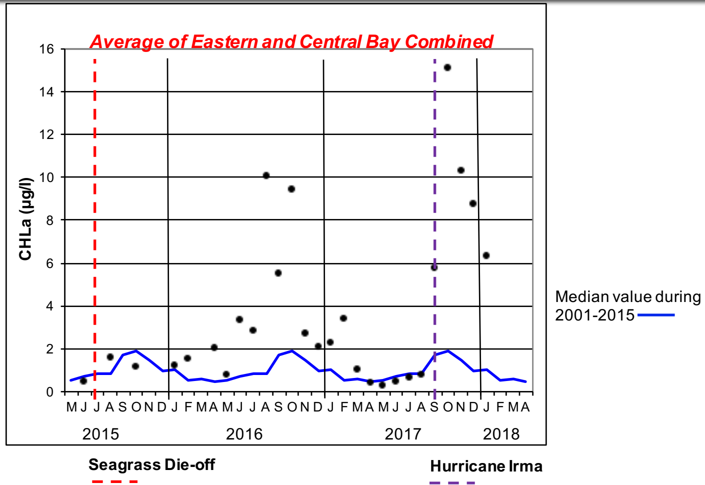
Figure 3. Average chlorophyll a (algal) concentrations in Florida Bay from 2015-2018 versus the historical average (blue line). Algal blooms in 2016 that were caused by nutrient releases from a large seagrass die-off in 2015 had subsided to background levels in 2017 until Hurricane Irma triggered a new bloom.
