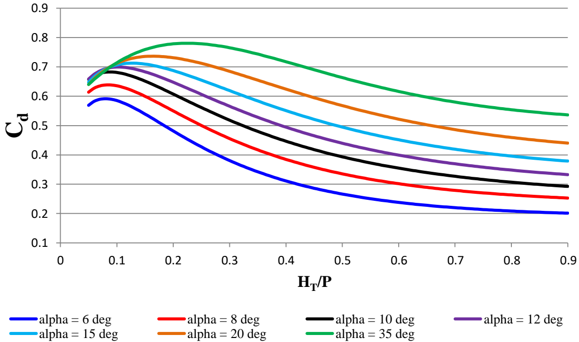
Figure D3. C_d vs. H_T/P (reconstructed from Crookston, 2010)
