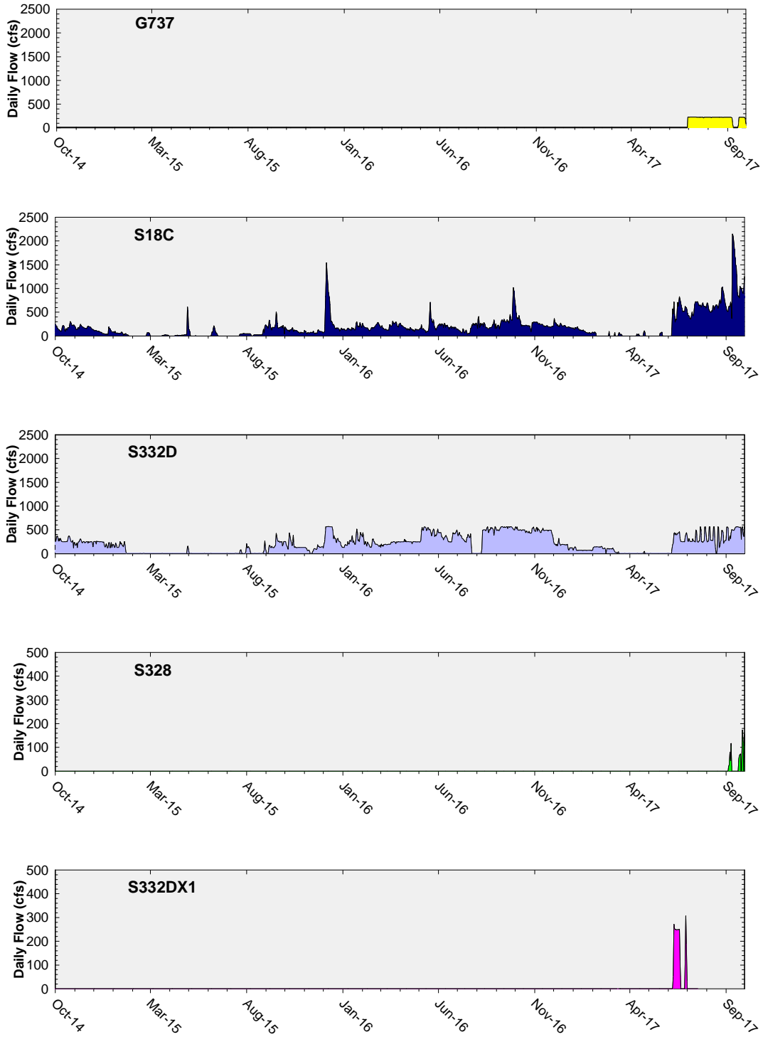
Figure 16. Daily flows at individual Taylor Slough and Coastal Basins structures into ENP.
