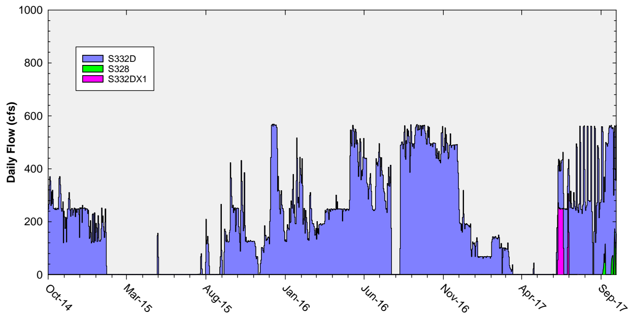
Figure 15. Overlaid daily flows from S332D pumps and at downstream structures.
