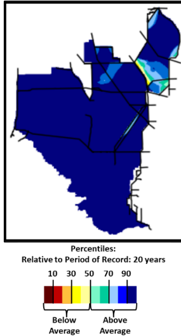
Figure EV-7. Present water depths (3/31/2024) compared to the day of year average over the previous 20 years.
