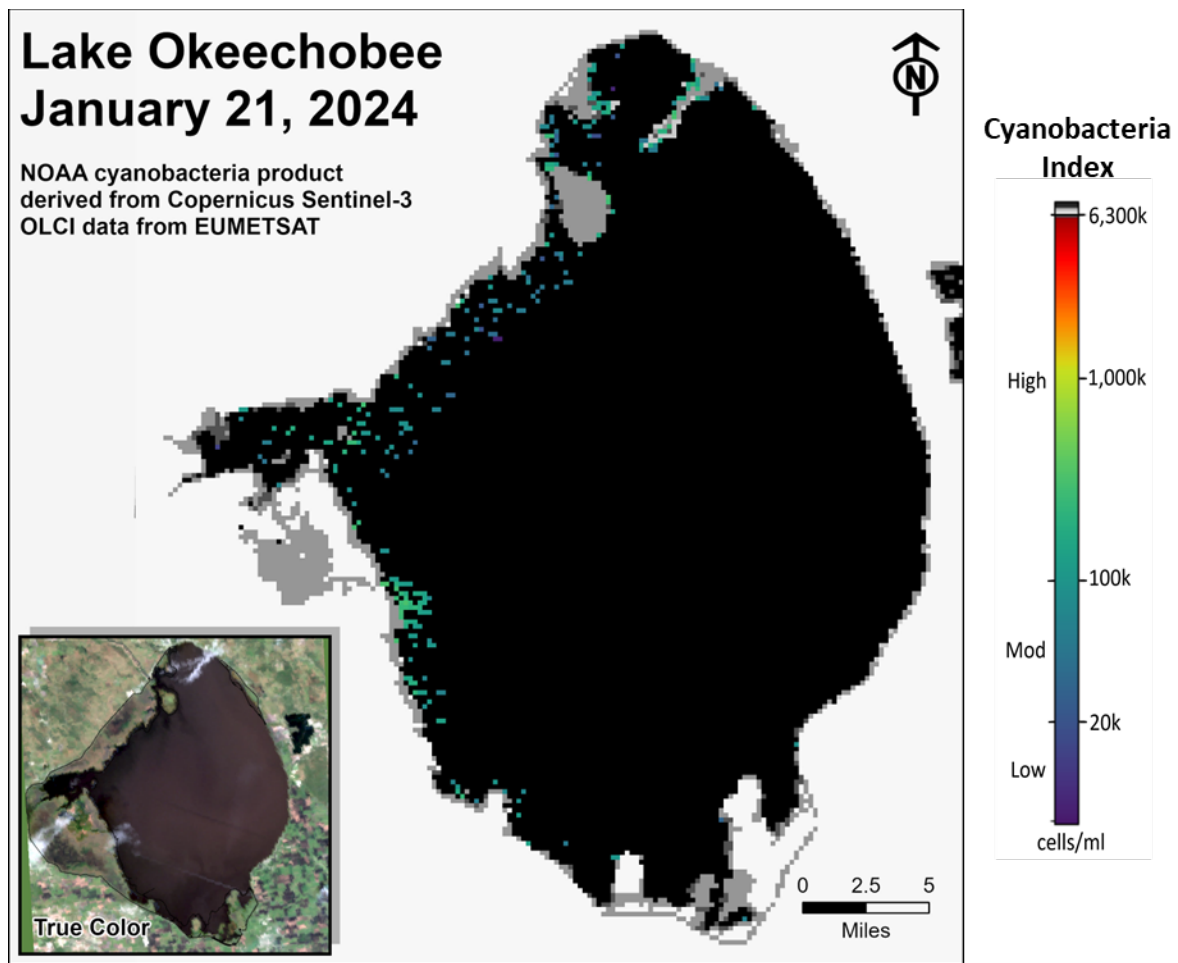
Figure LO-7. Cyanobacteria bloom index level on January 21, 2024, based on NOAA’s harmful algal bloom monitoring system. Gray color indicates cloud cover.
