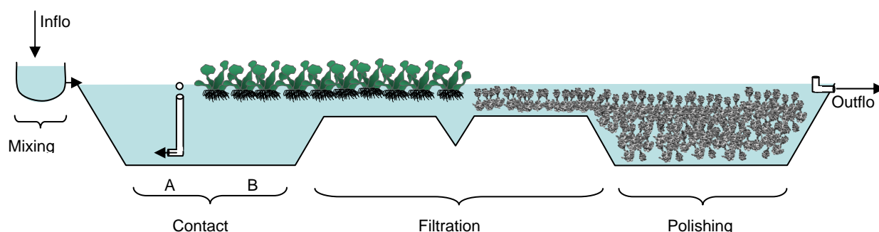
Figure 6.1-4. Typical Hybrid Wetland Treatment Technology
