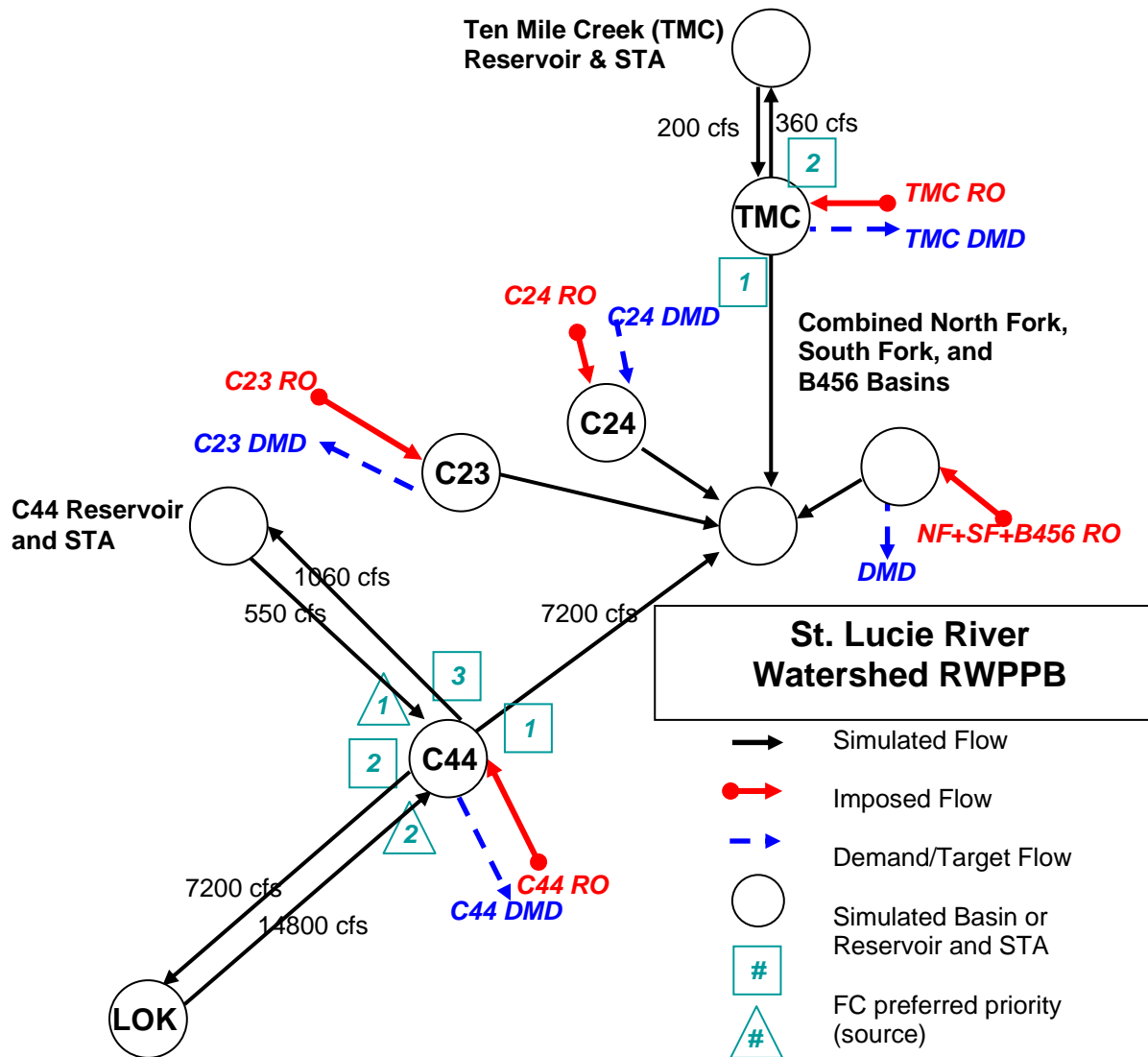
Figure 6.2-2. St. Lucie River Watershed Simulation Configuration for RWPPB
