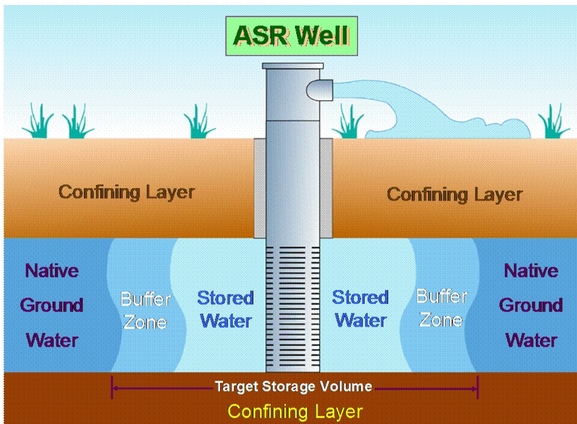
Figure 6.1-1. Typical Aquifer Storage and Recovery Well System
