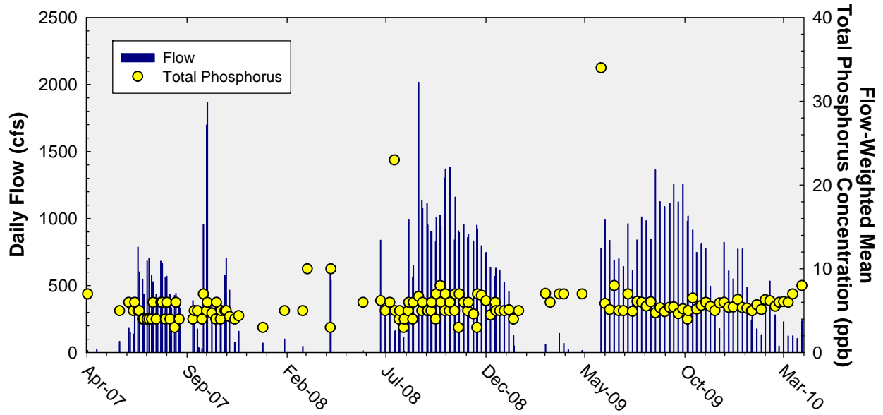
Figure 15. Total daily flow from Taylor Slough and Coastal Basins structures (S332D + S174 and S18C) and the corresponding flow-weighted mean total phosphorus concentrations for individual sampling events.
