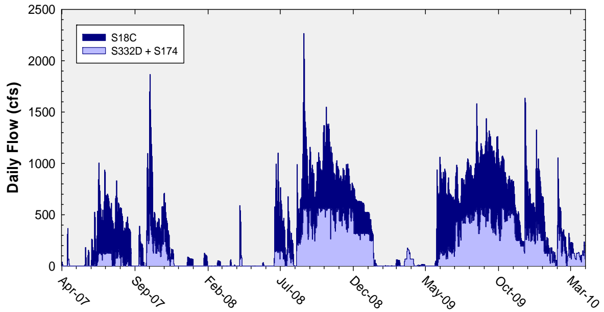
Figure 13. Daily flows into Everglades National Park as a stacked sum of Taylor Slough (structures S332D + S174) and Coastal Basins (structure S18C). Structure S174 was plugged in September 2007 and is no longer used.
