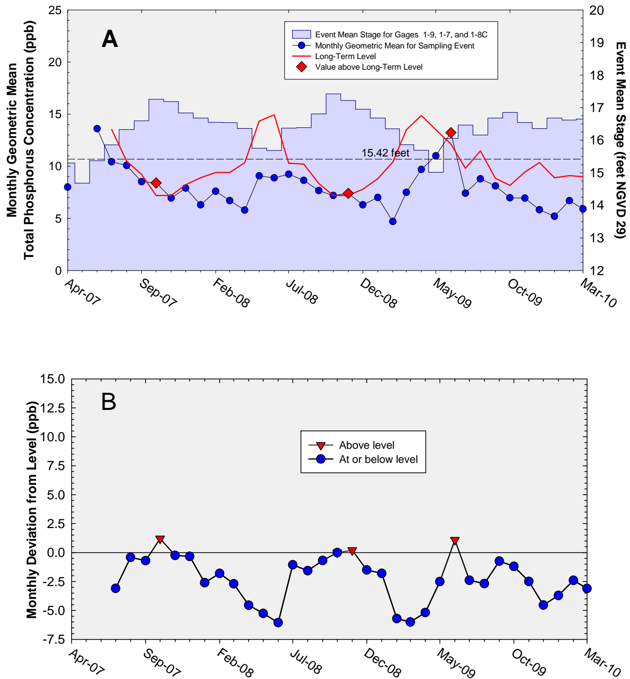
Figure 3. (A) Monthly total phosphorus geometric mean concentrations for the Arthur R. Marshall Loxahatchee National Wildlife Refuge compared to calculated long-term levels. These calculated long-term total phosphorus levels are adjusted for fluctuations in stage. The long-term levels were not applicable for April 2007 through June 2007 because the average stage was less than 15.42 feet. The geometric mean was greater than the long-term level in October 2007, November 2008, and June 2009.
