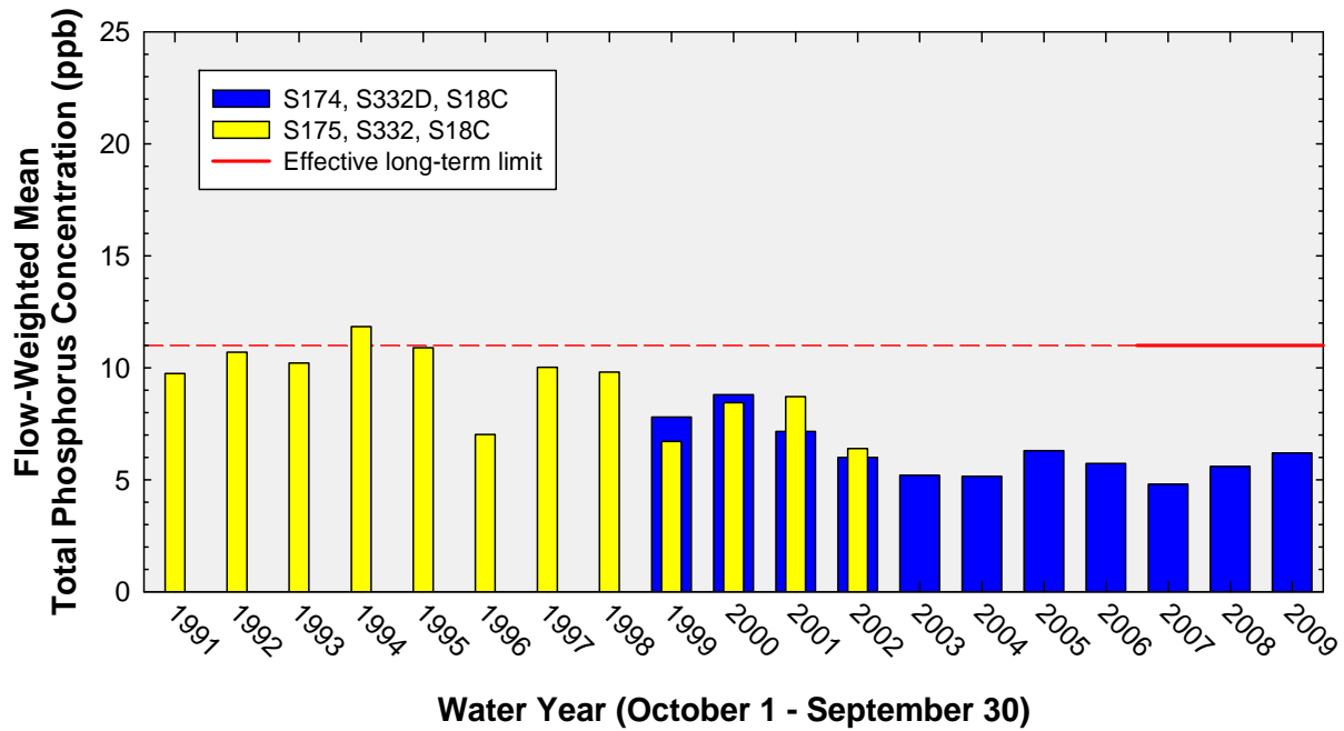
Figure 11. The 12-month flow-weighted mean total phosphorus concentrations in inflows to Everglades National Park through Taylor Slough and Coastal Basins at the end of each water year compared to the 11 ppb long-term total phosphorus limit.
