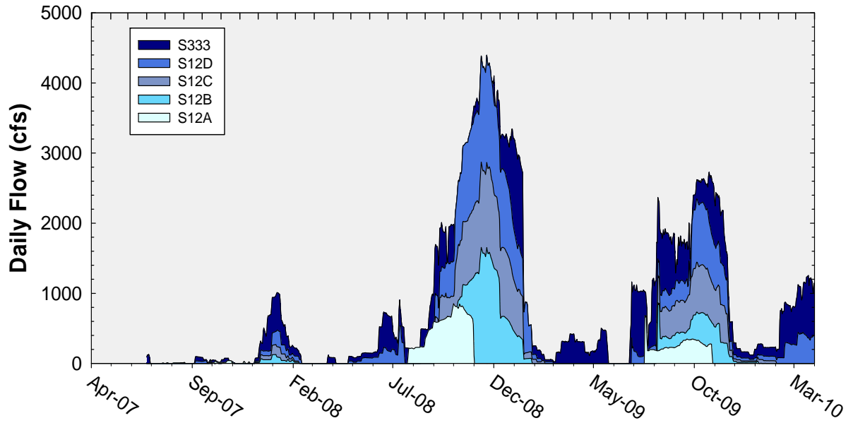
Figure 7. Daily flows at Shark River Slough structures as a stacked sum of five inflows.
