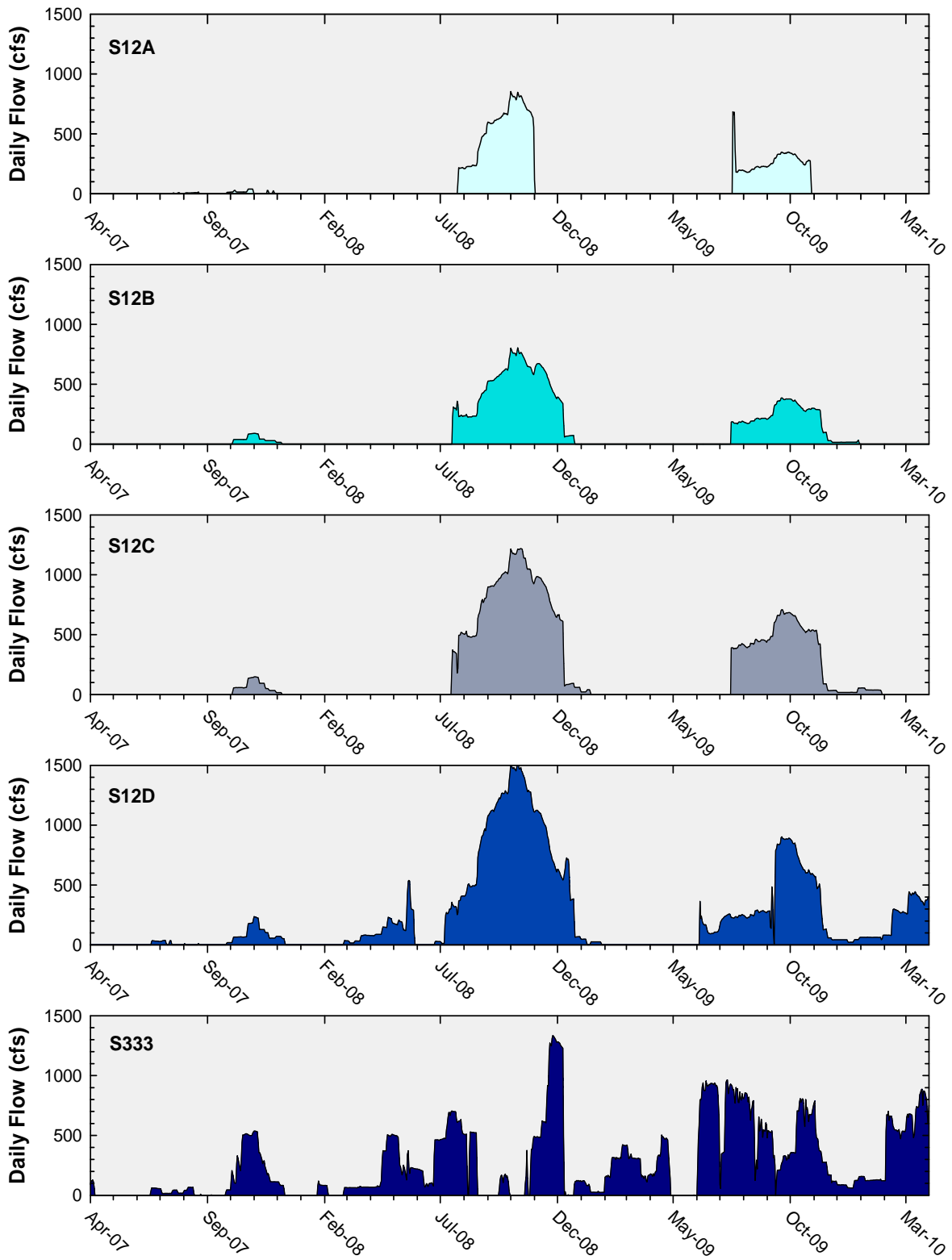
Figure 9. Daily flows at individual inflow structures to Shark River Slough. This figure includes most of the data illustrated in Figures 7 and 8.
