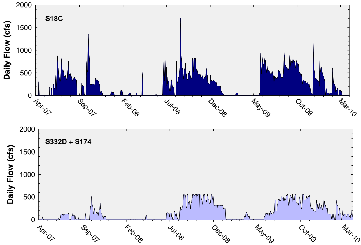
Figure 14. Daily flows at individual Coastal Basins (S18C) and Taylor Slough (S332D + S174) structures into the Everglades National Park.
