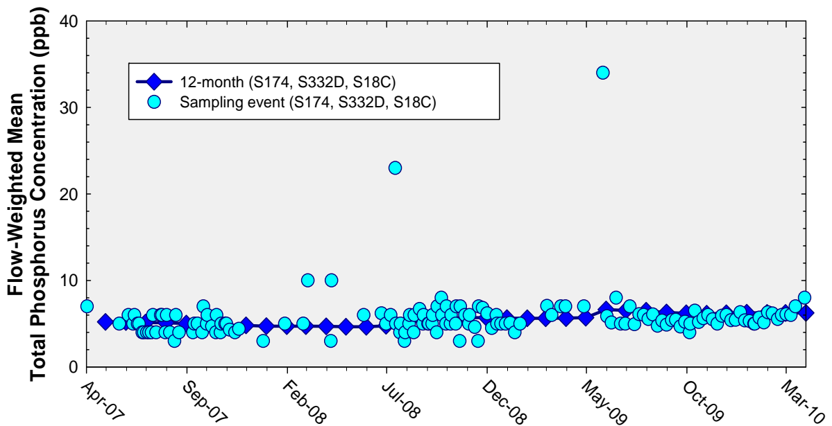
Figure 12. The 12-month flow-weighted mean total phosphorus concentrations in inflows to Everglades National Park through Taylor Slough and Coastal Basins at the end of each month and the flow-weighted mean total phosphorus concentration for each sampling event.
