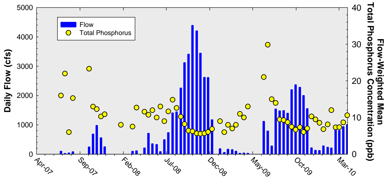
Figure 10. Total daily flow at Shark River Slough structures and the corresponding flow-weighted mean total phosphorus concentrations for individual sampling events.
