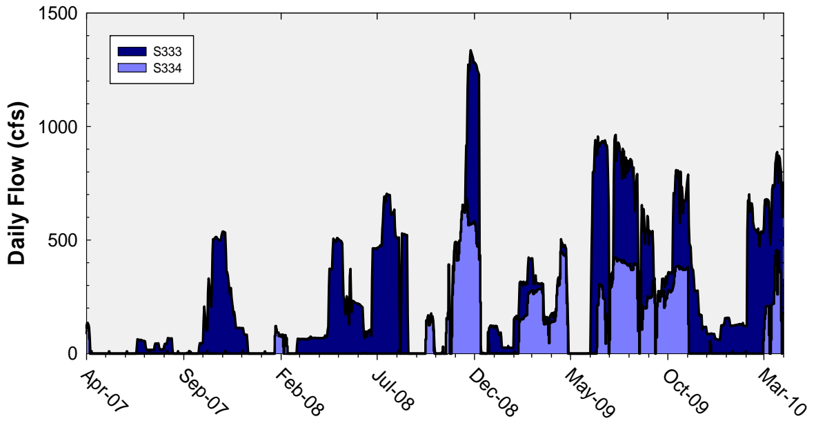
Figure 8. Daily flows at structures S333 and S334.
