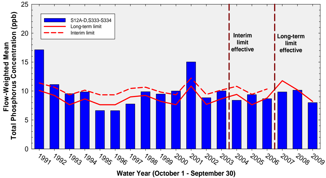
Figure 5. The 12-month flow-weighted mean total phosphorus concentrations at inflows to the Everglades National Park through Shark River Slough at the end of each water year compared to the interim and long-term total phosphorus limits. The 12-month flow-weighted mean concentrations have met the interim limits since they became effective on October 1, 2003. The 12-month flow-weighted mean TP concentration for the compliance year through September 30, 2009, was 8.2 ppb and was equal to the long-term limit.
