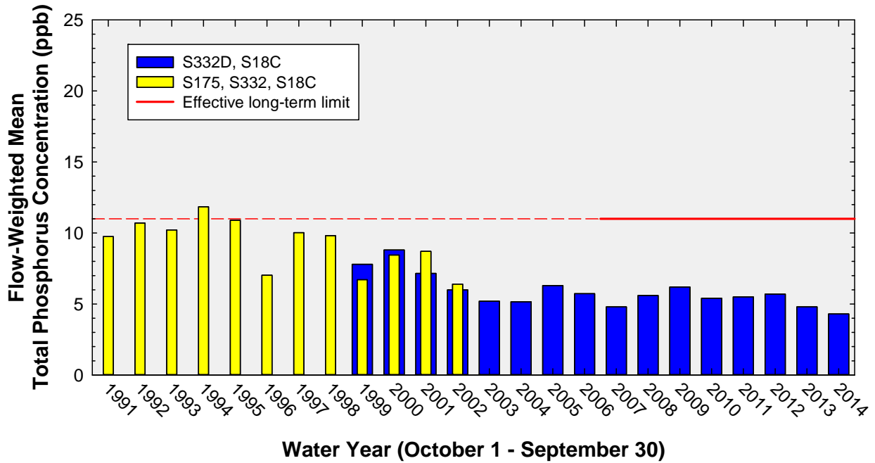
Figure 5. The 12-month flow-weighted mean TP concentrations in inflows to ENP through Taylor Slough and Coastal Basins at the end of each water year compared to the 11 ppb long-term TP limit.
