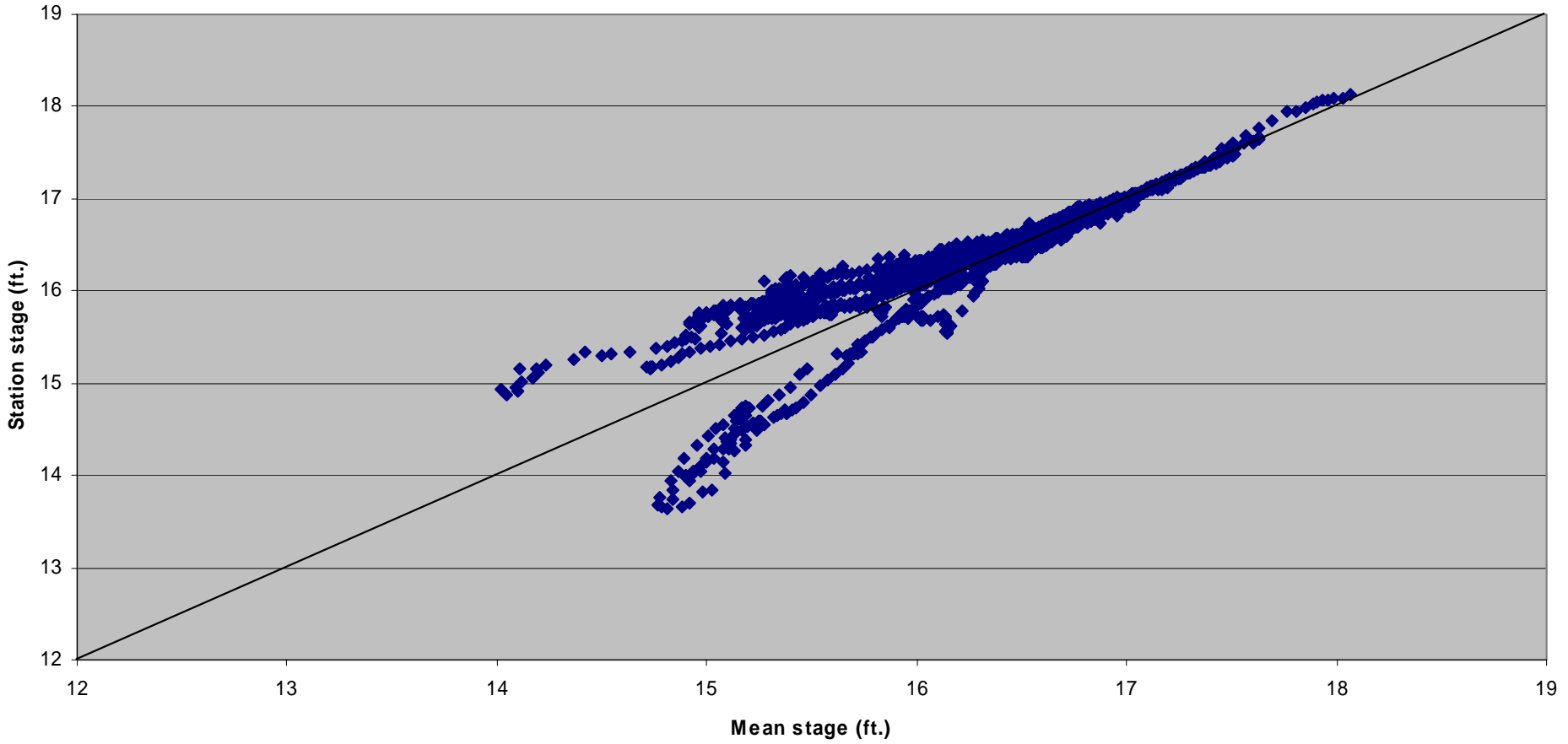
1-7 Station Stage versus Mean Stage
