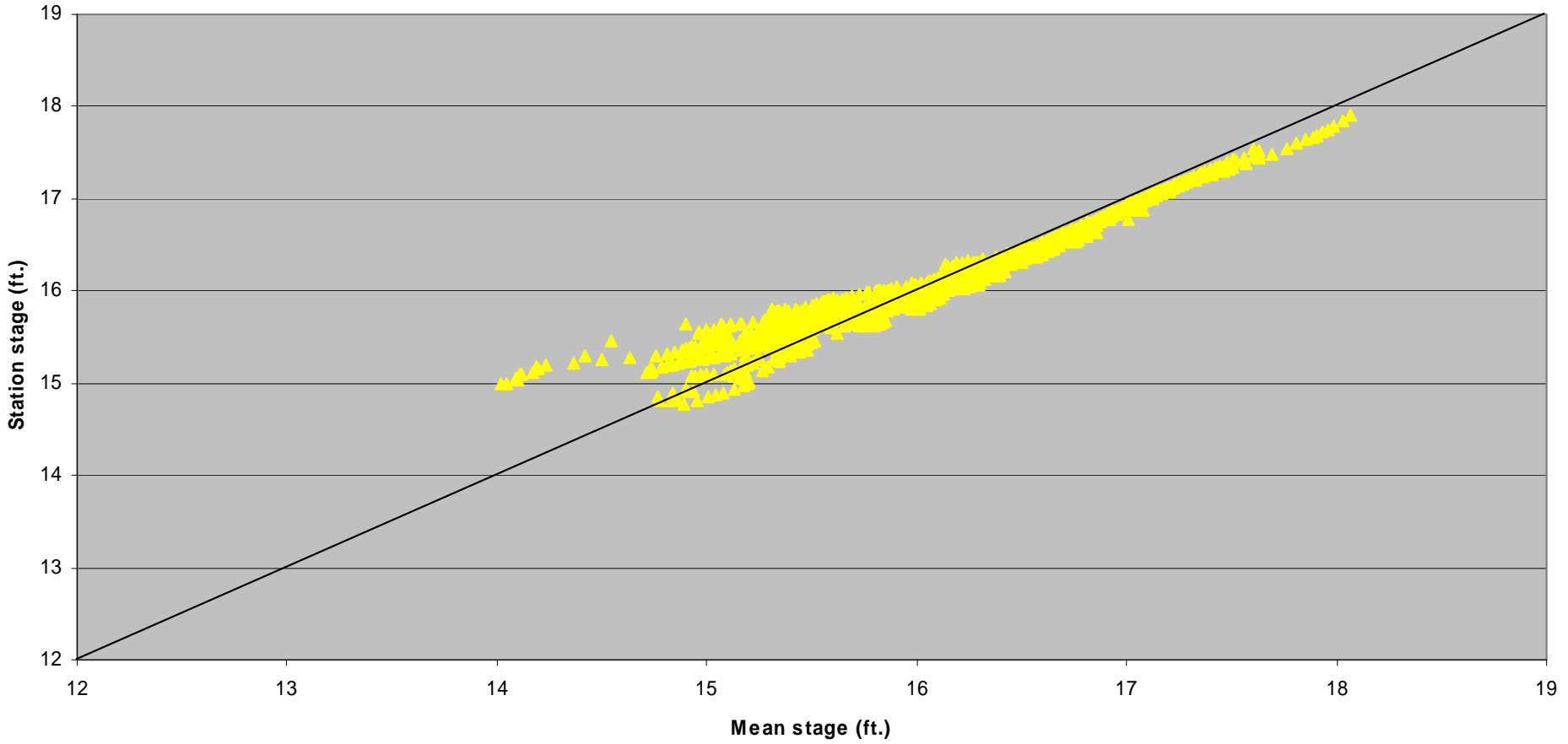
1-9 Station Stage versus Mean Stage
