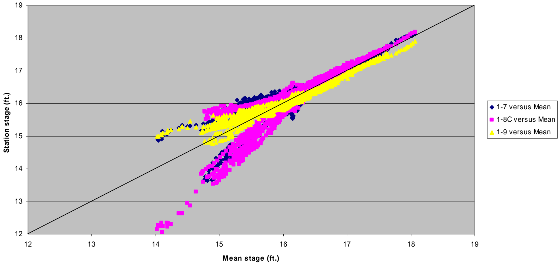
Station Stage versus Mean Stage
