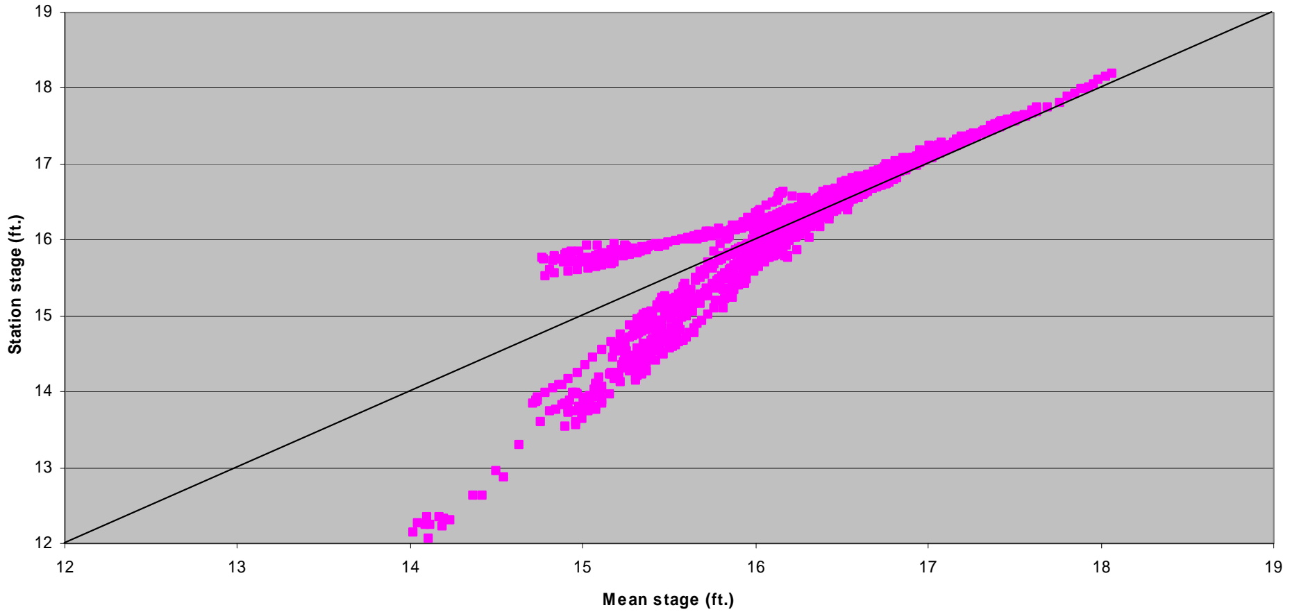
1-8C Station Stage versus Mean Stage
